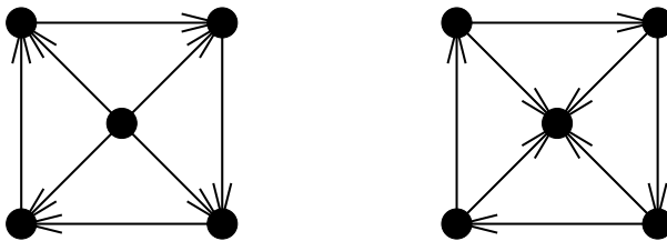
Figure 6.12: These two graphs cannot be distinguished by the principle eigenvalue method.
