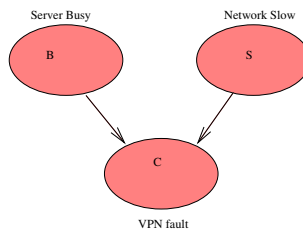
Figure 17.2: A simple Bayesian network with two possible cause hypotheses.
