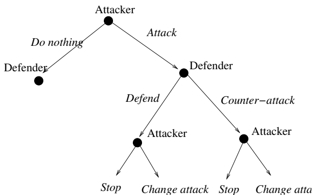
Figure 19.1: The extensive form of a game is a complete history of the state space of the players. By tracing the choices made from the start of the game, a player can examine the payoff accrued and predict the best course of action for the remaining moves.
