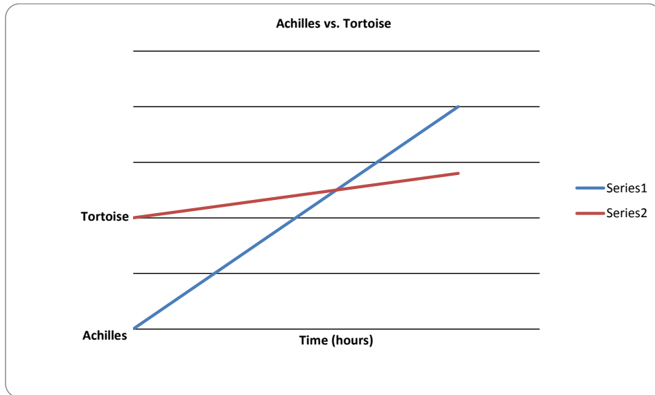
Figure A.5 Achilles racing the Tortoise.
