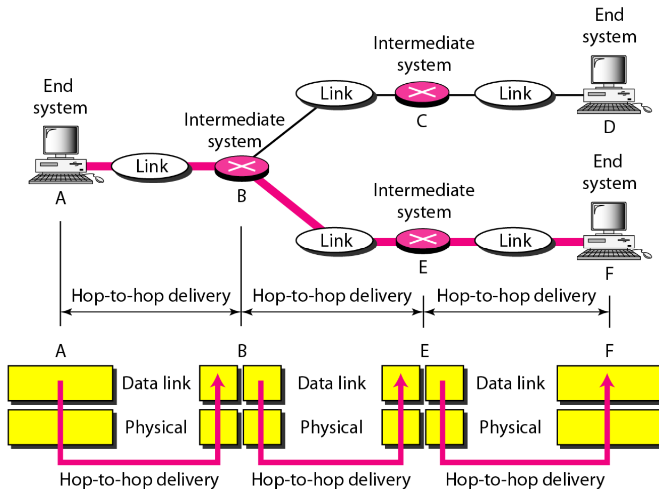
Figure 2.7 Hop-to-hop delivery
