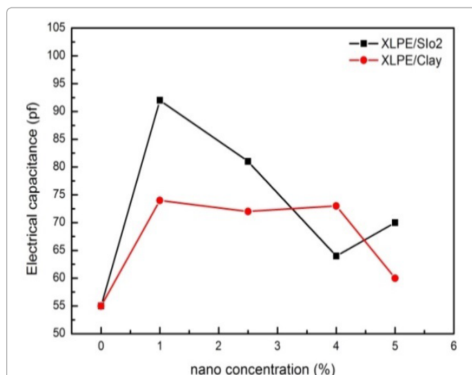
Figure 10: Histogram illustrates the comparison between electric capacitance of the XLPE which modified with SiO 2 nanofiller and XLPE which modified with clay nanofiller.
