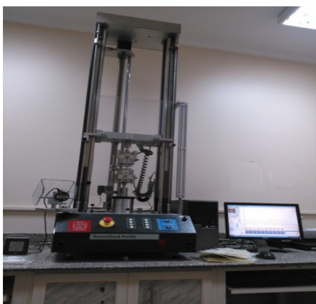
Figure 7: Mechanical measurements tester, (BS EN 60811).
