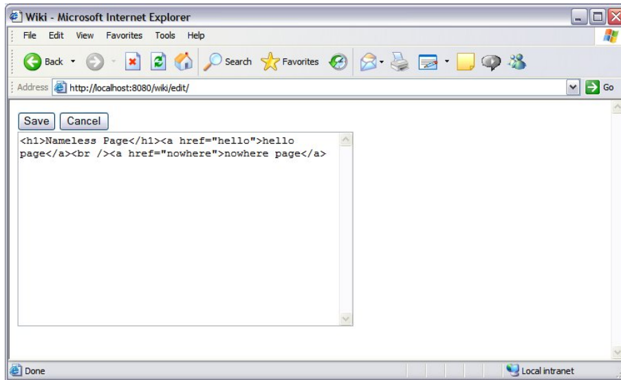
Figure 15.16: Edit Page
