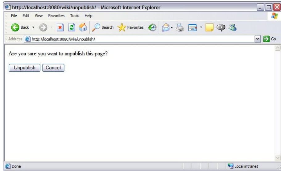
Figure 15.24: Unpublish Page
