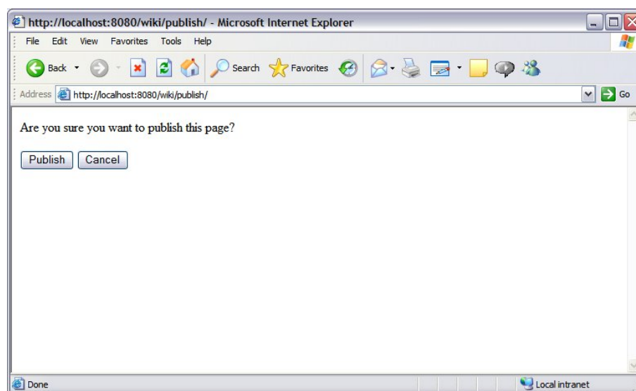
Figure 15.19: Publish Page
