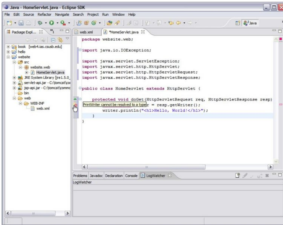
Figure 5.9: Error message
