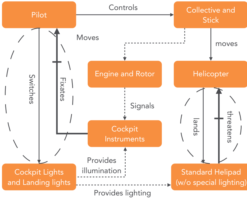
Figure 20. Function diagram of the helipad system
