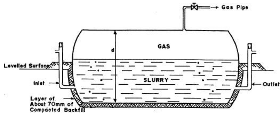
Figure (4.8): Bag digester [34].
