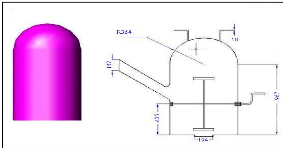
Figure (7.1): Sketch of a family digester in Palestine ( 0.5 \text{ m}^3 )
