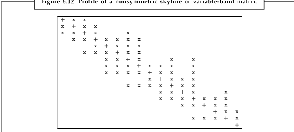
Figure 6.12: Profile of a nonsymmetric skyline or variable-band matrix.
