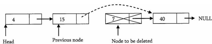
Figure 8.12: Dispose the current node
