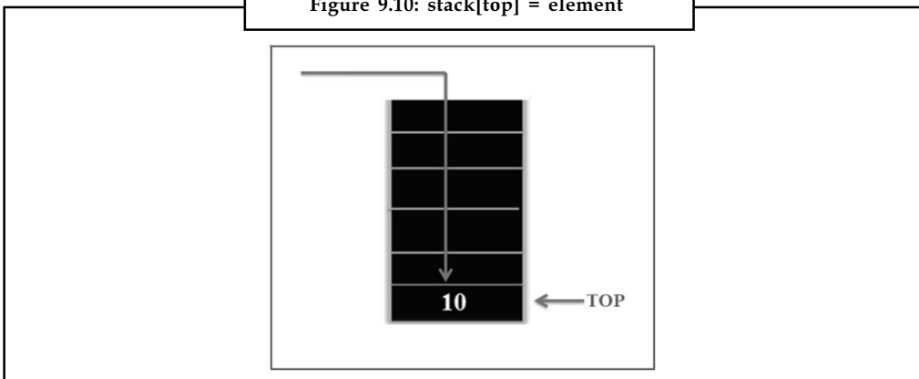
Figure 9.10: stack[top] = element
