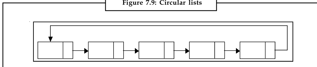
Figure 7.9: Circular lists
