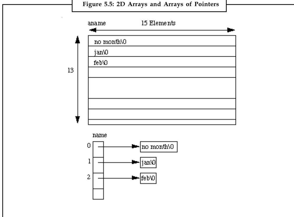
Figure 5.5: 2D Arrays and Arrays of Pointers
