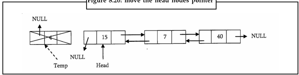
Figure 8.20: move the head nodes pointer
