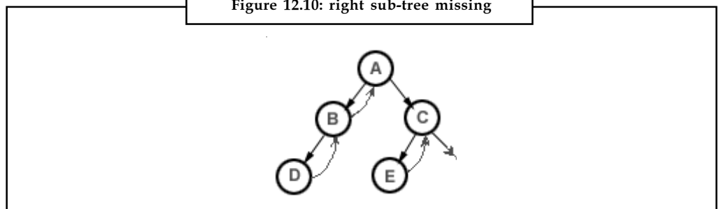
Figure 12.10: right sub-tree missing
