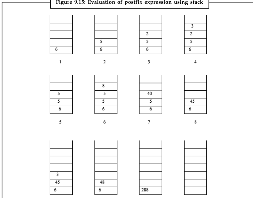
Figure 9.15: Evaluation of postfix expression using stack
