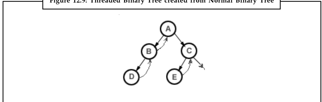
Figure 12.9: Threaded Binary Tree created from Normal Binary Tree
