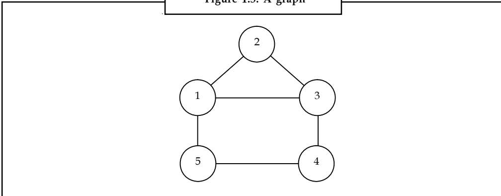
Figure 1.5: A graph
