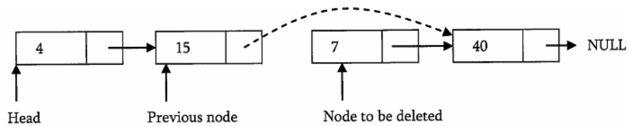
Figure 8.11: change the previous nodes next pointer to next pointer of the node to be deleted
