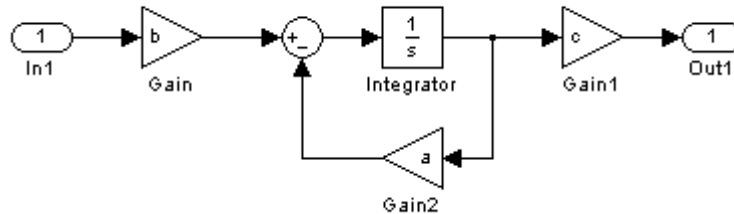
Figure 10.2 Diagram of Model for One State Variable.
