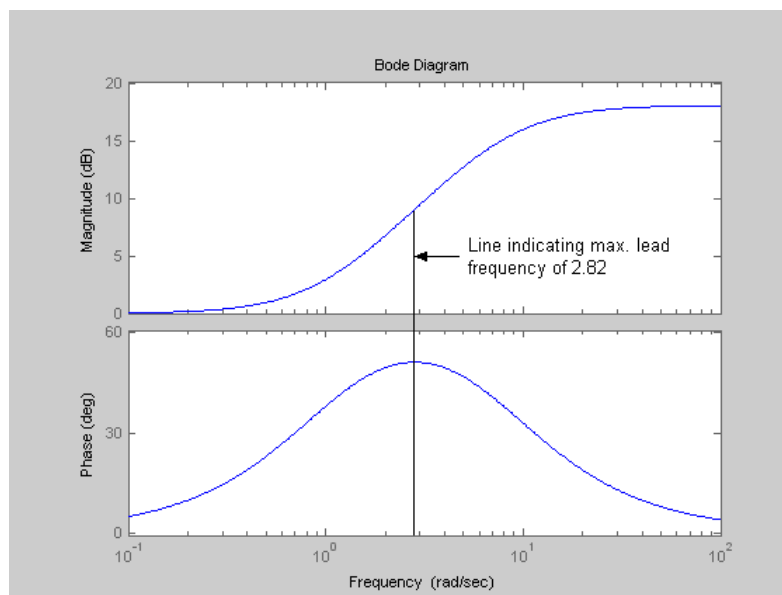
Figure 7.1 Bode diagram of phase lead with T = 1 and \alpha = 1/8 .
