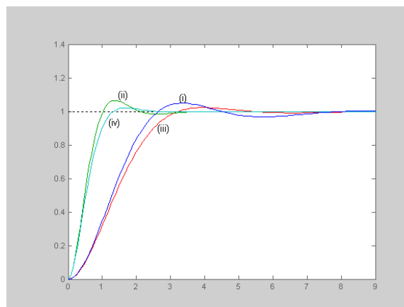
Fig.11.2 Responses for example 1 for ISTE (i) and (ii); IST 2 E (iii) and (iv)
