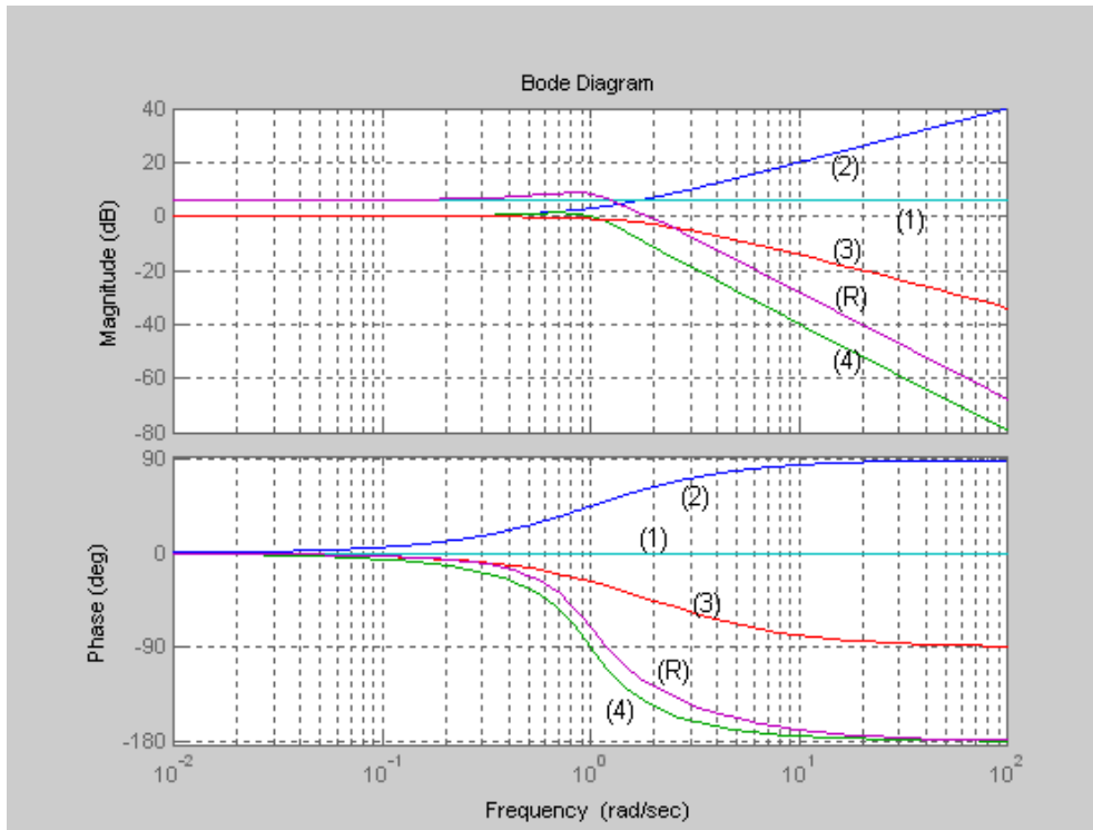
Figure 4.3 Bode plot of G(s) of equation (4.10) and its constituents.
