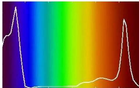
Figure 4.5 Absorption spectrum of a typical plant
