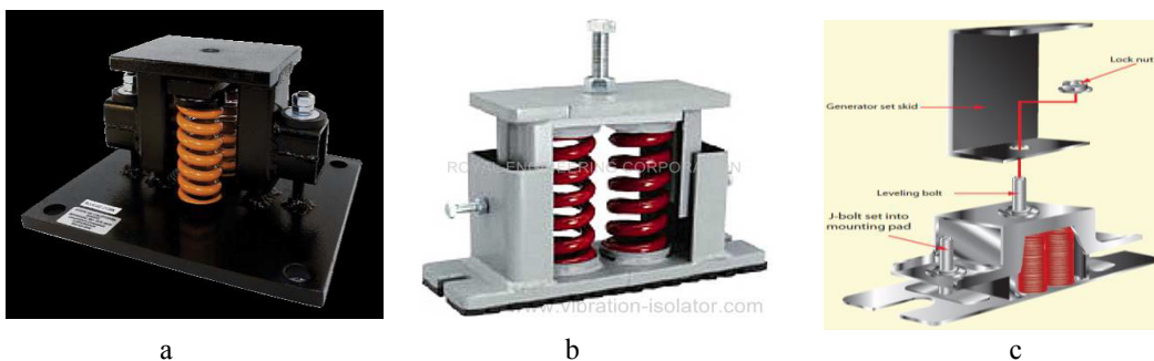
Figure 11: Different forms of spring isolator.
