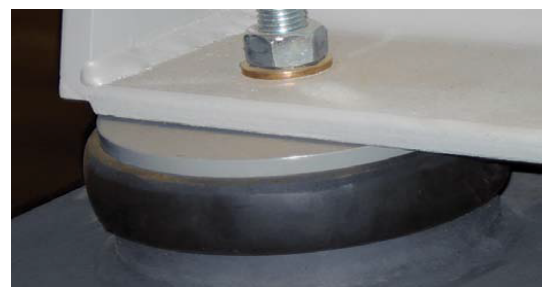
Figure 8: An elastomeric isolator between the generator foot and base minimizes the transfer of energy to the base.
