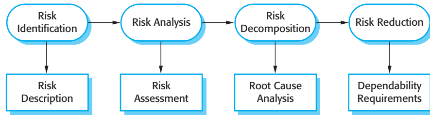
Figure 12.1 Risk-driven specification
