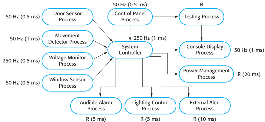
Figure 20.16 Alarm process timing
