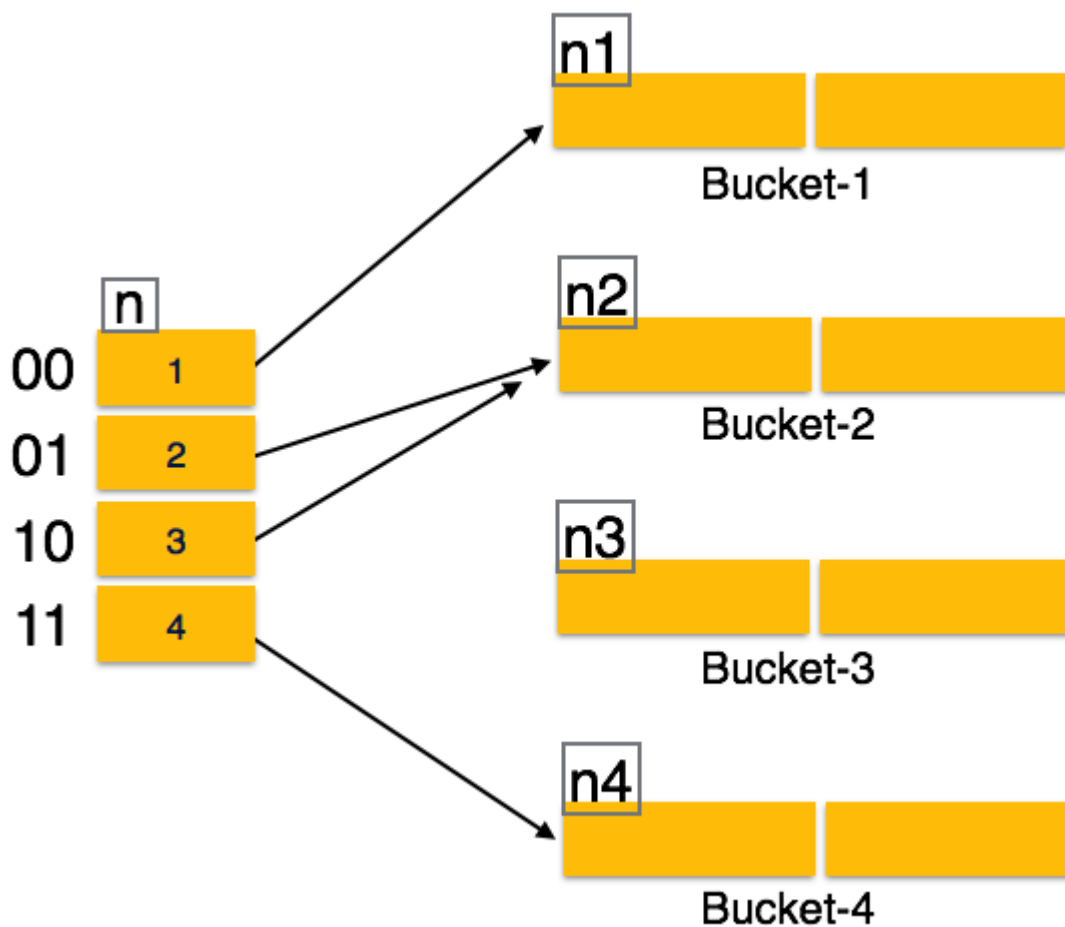
[Image: Dynamic Hashing]
