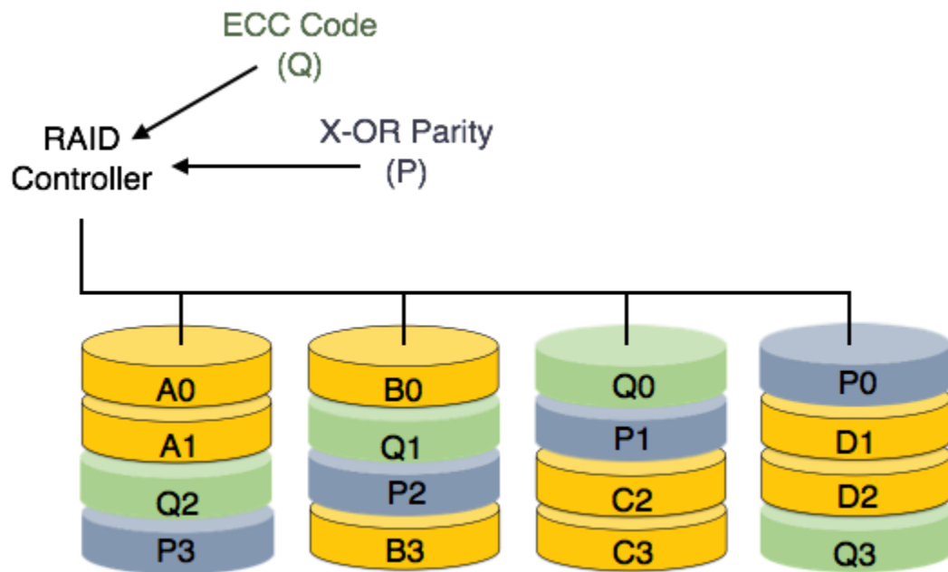
[Image: RAID 6]
