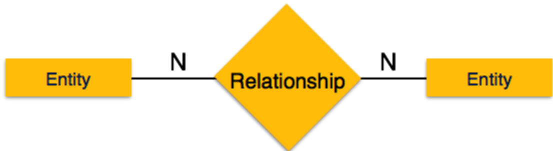
[Image: Many-to-many]
