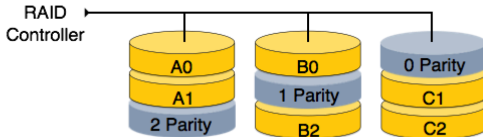
[Image: RAID 5]
