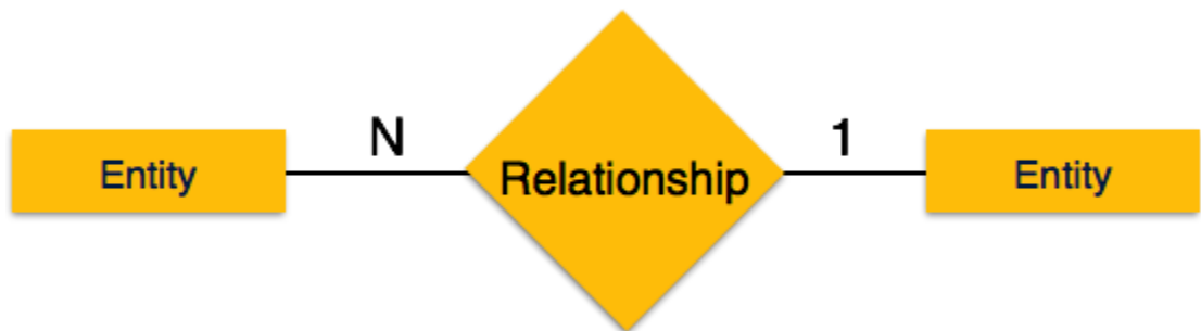
[Image: Many-to-one]
