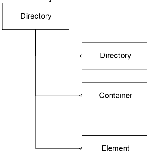
Fig. 3 Metadirectory content
