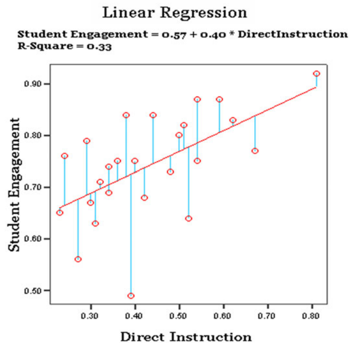
Figure 1. Linear models approach to measuring a relation
