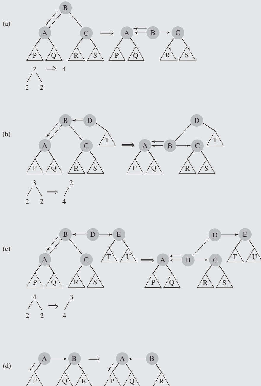
FIGURE 7.31 Deleting a node from a vh-tree.
