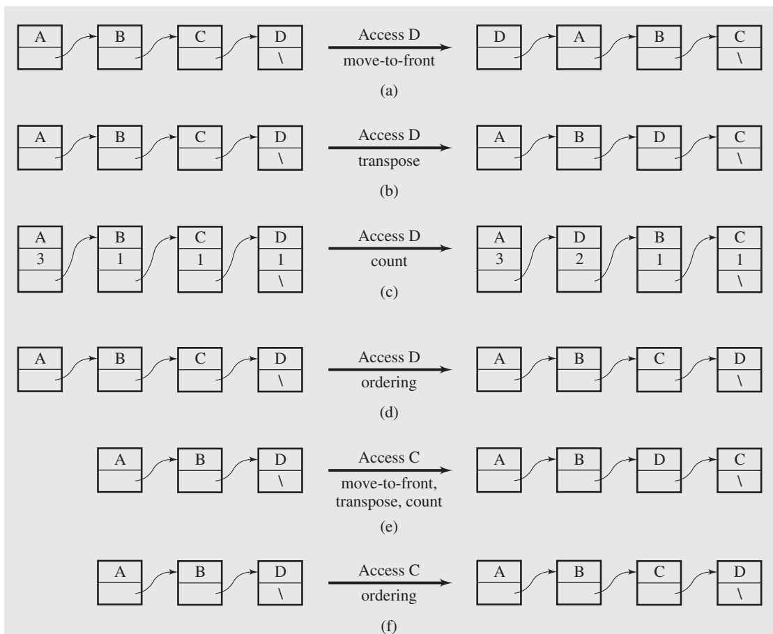
FIGURE 3.18 Accessing an element on a linked list and changes on the list depending on the self-organization technique applied: (a) move-to-front method, (b) transpose method, (c) count method, and (d) ordering method, in particular, alphabetical ordering, which leads to no change. In the case when the desired element is not in the list, (e) the first three methods add a new node with this element at the end of the list and (f) the ordering method maintains an order on the list.
