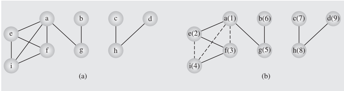
FIGURE 8.3 An example of application of the depthFirstSearch() algorithm to a graph.
