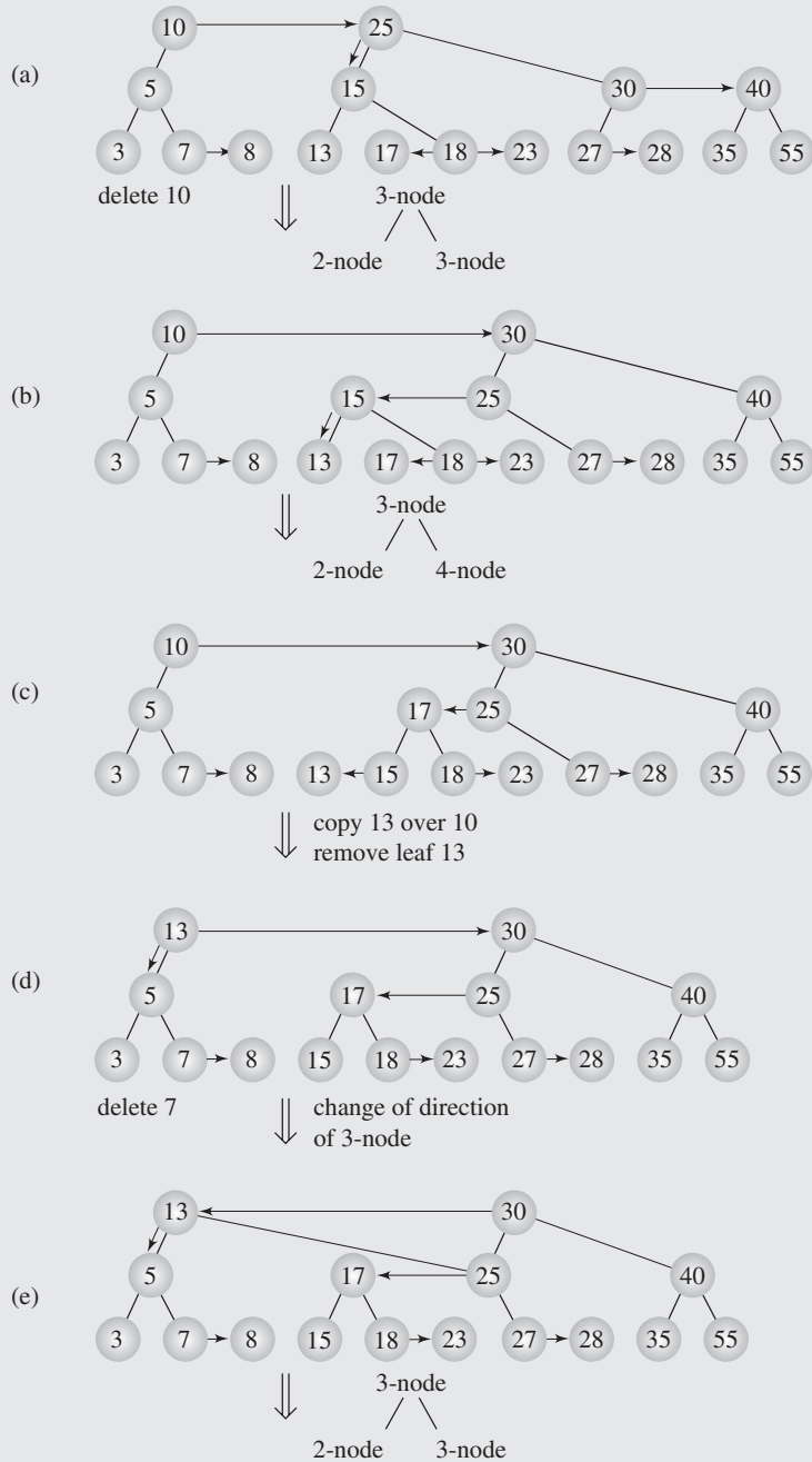
FIGURE 7.32 Examples of node deletions from a vh-tree.
