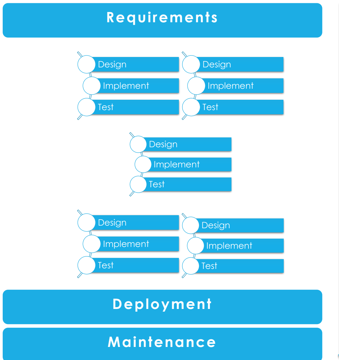
Figure 4 - Iterative Approach
