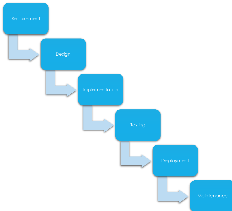
Figure 2 - Waterfall Approach
